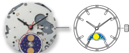
6P24 Height 3.45mm 1 eye (Moon) 3 year battery life (SR621SW)
