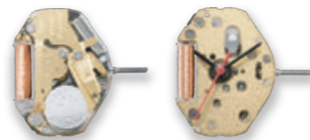
Super 2035 Height 3.15mm 4 year battery life (SR626SW)
