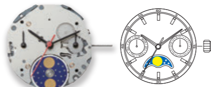
6P20 Height 3.45mm 3 eyes (Day/Date/Moon) 3 year battery life (SR621SW)
