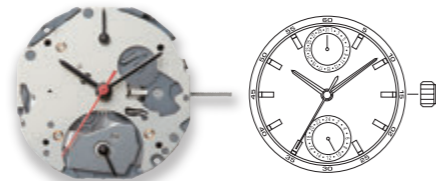
6P23 Height 3.45mm 2 eyes (Date/24 hour) 3 year battery life (SR621SW)
